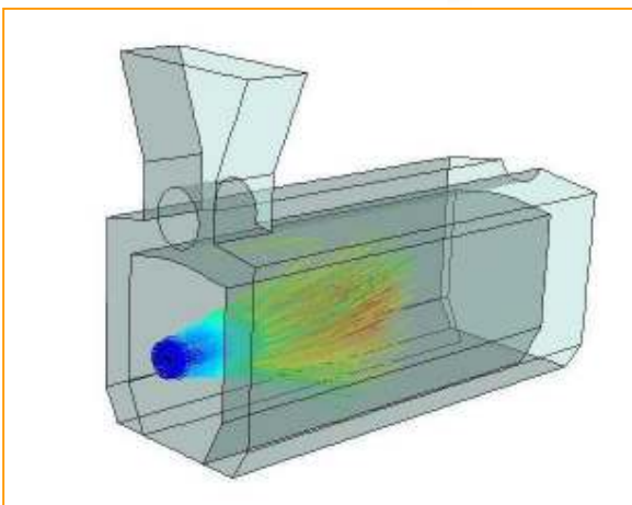
Figure shows the model of an Industrial Boiler for CFD simulations and the flame propagation inside the boiler.
